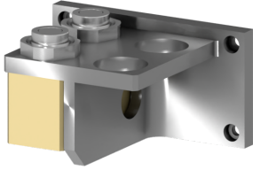
Coolant module IN/OUT with 4 fittings M20x1.5.
