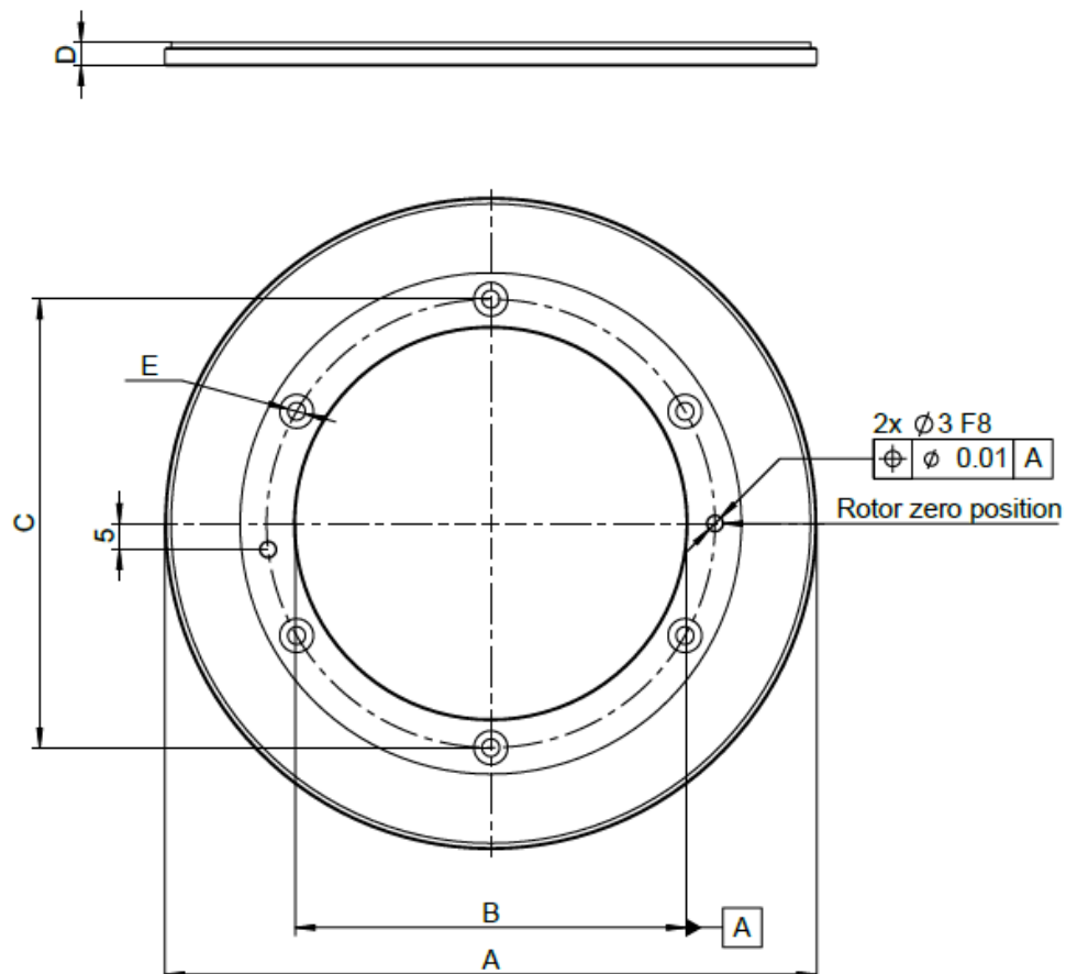
Inductive MAX Encoder - Rotor IMR-125 anodized aluminum
