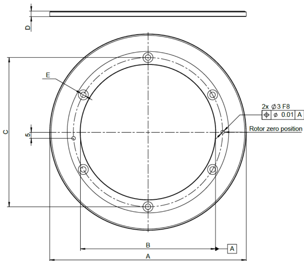
Inductive MAX Encoder - Rotor IMR-180 anodized aluminum
