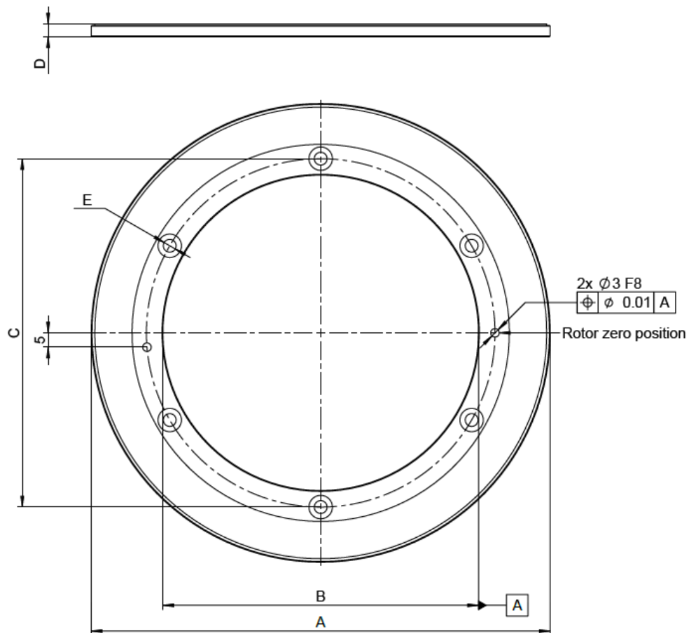
Inductive MAX Encoder - Rotor IMR-160 anodized aluminum
