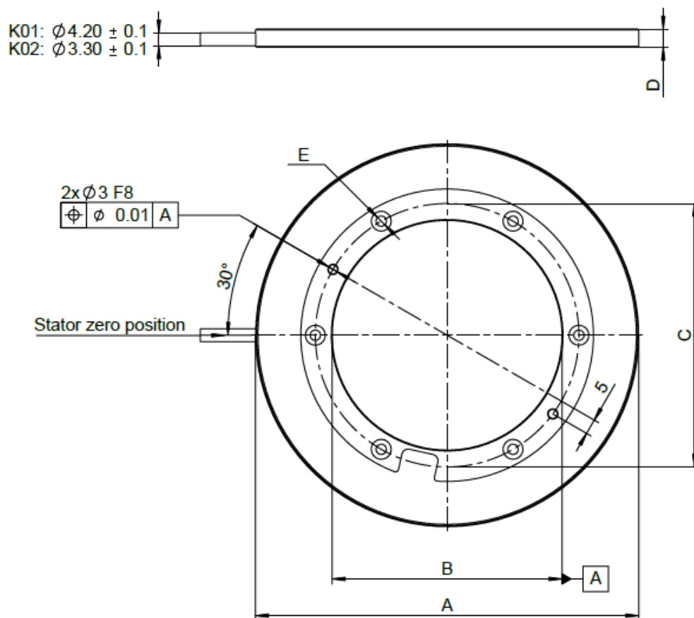
Inductive MAX Encoder - Stator IMS-125 anodized aluminum
